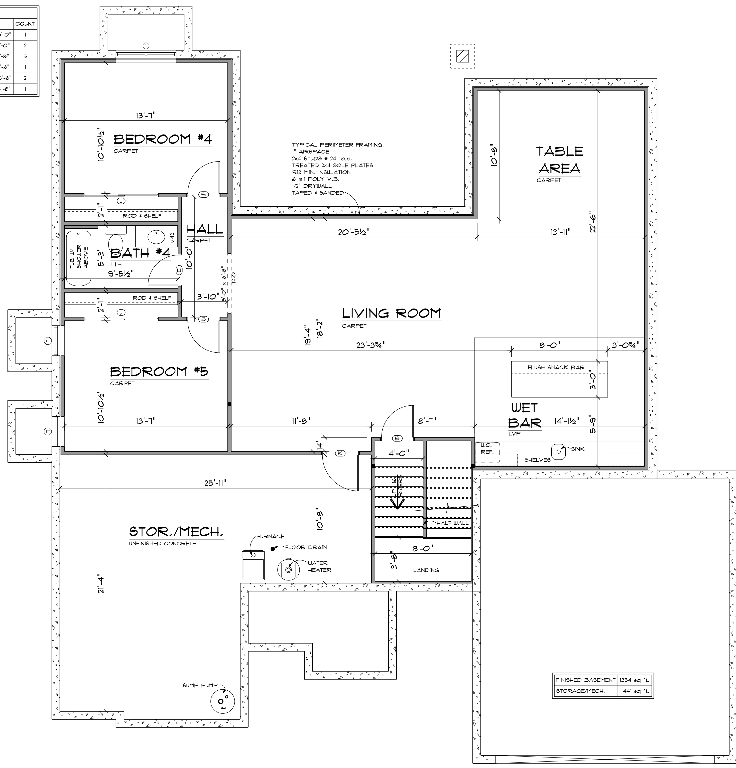
FINISHED BASEMENT PLAN SCALE: 1/4" = 1'-0"
